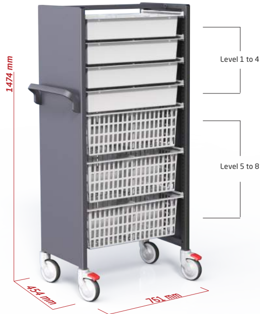
Delivery cart with divider tray
