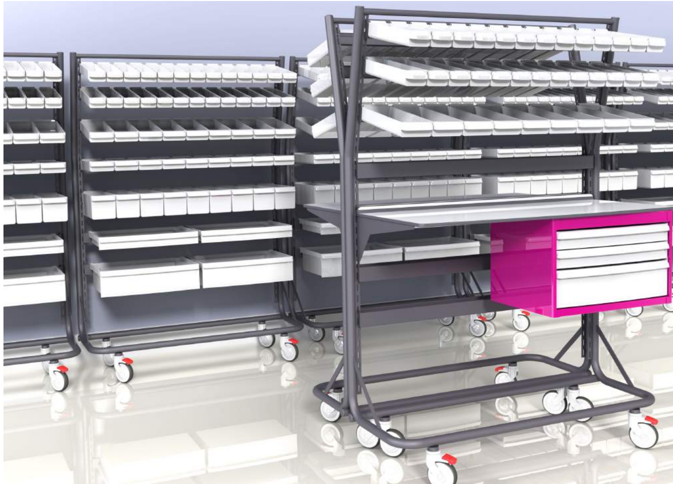
Suggestion for picking station area layout
