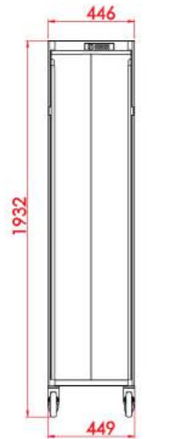
Logist'Alli F400 20G
