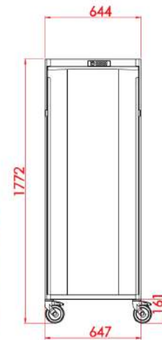
Logist'Alli F600 18G
