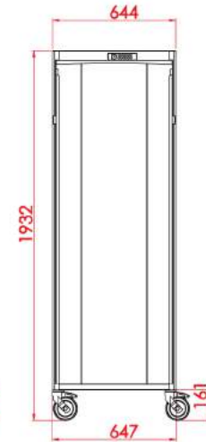
Logist'Alli F600 20G
